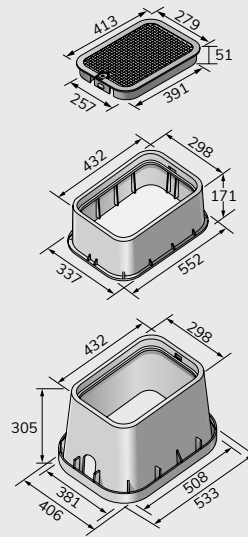
14" x 19" Rectangular Valve Boxes
